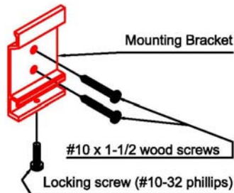
Figure 1 Wall Mounted
