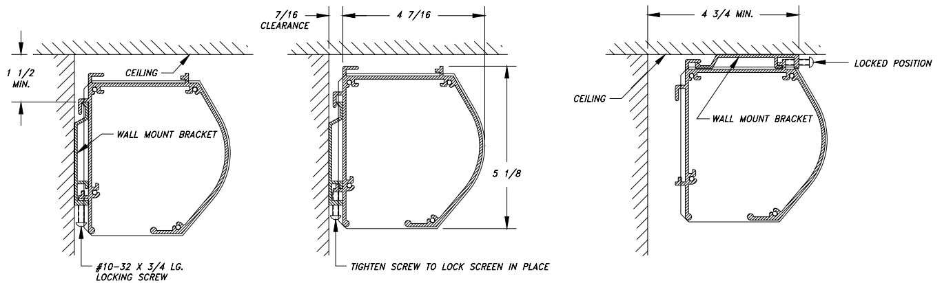
Figure 1 Wall Mounted
